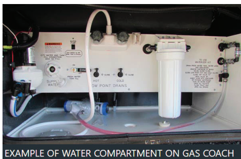
EXAMPLE OF WATER COMPARTMENT ON GAS COACH
