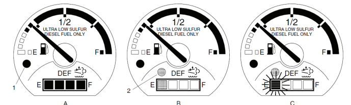
11/08/2010 A. Green bars—DEF level indicators B. One bar illuminated amber—DEF very low, refill DEF C. One bar flashing red—DEF empty, refill DEF 1. Low Fuel Warning Lamp 2. DEF Warning Lamp 1611037
