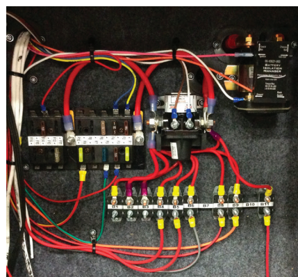
Shore Power Compartment Fuse Example
