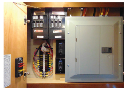
Diesel Pusher Fuse Panel Example
