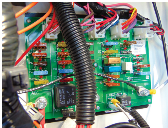
Example of a KIB Fuse Panel
