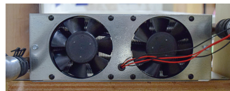
Oasis Dual Fan on Basement Heat Exchanger
