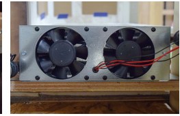
Oasis Dual Fan on Basement Heat Exchanger
