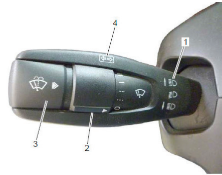
02/17/2017 1. Headlight Control Symbols 2. Windshield Wiper Switch 3. Windshield Washer Switch 4. Turn Signal Symbol f611264
