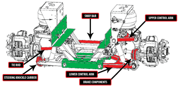
The chassis frame and suspension cradle (shown in green) are the proper lift points for towing.
