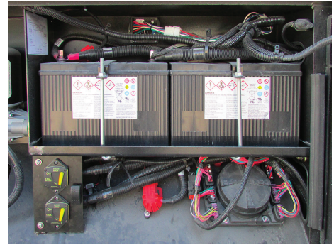
Spartan Chassis Fuse Panel Example
