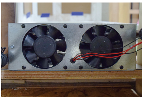
Oasis Dual Fan on Basement Heat Exchanger
