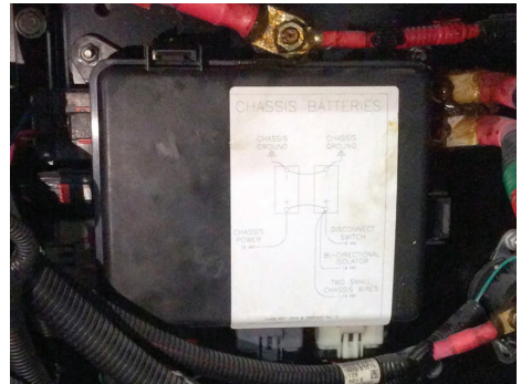
Freightliner Chassis Fuse Panel Example
