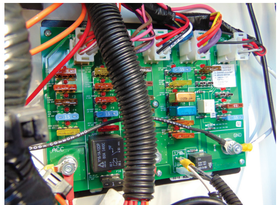
Example of a KIB Fuse Panel
