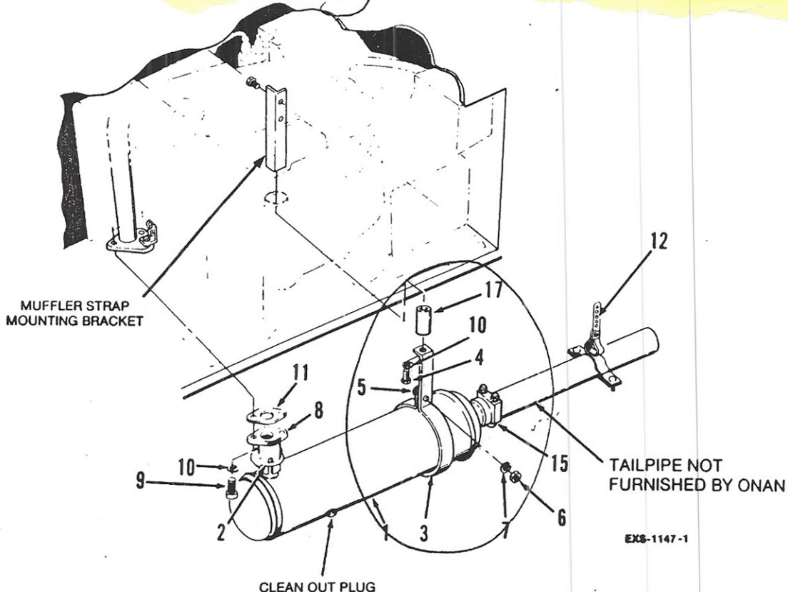
FIGURE 3. EMERALD I AND EMERALD III RIGHT EXHAUST INSTALLATION (KITS 542-0472, 542-0484, 154-2697)
