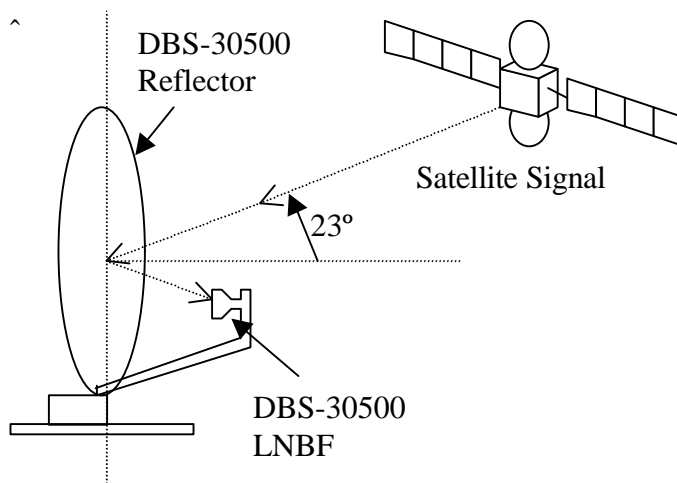
Figure 3. Signal Path Relative to Dish
