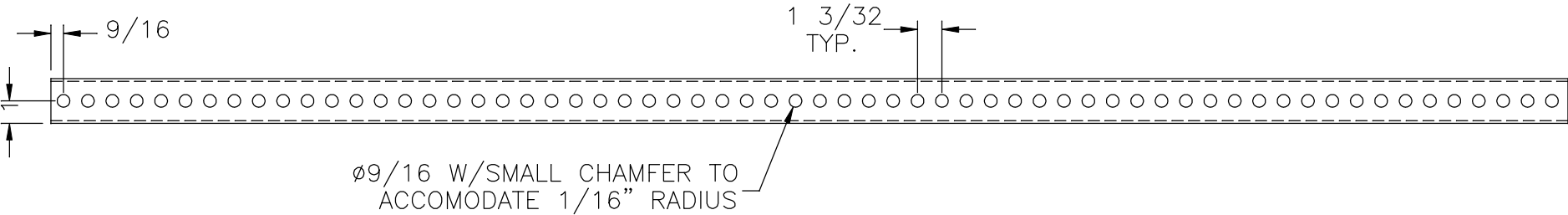
BOTTOM VIEW
