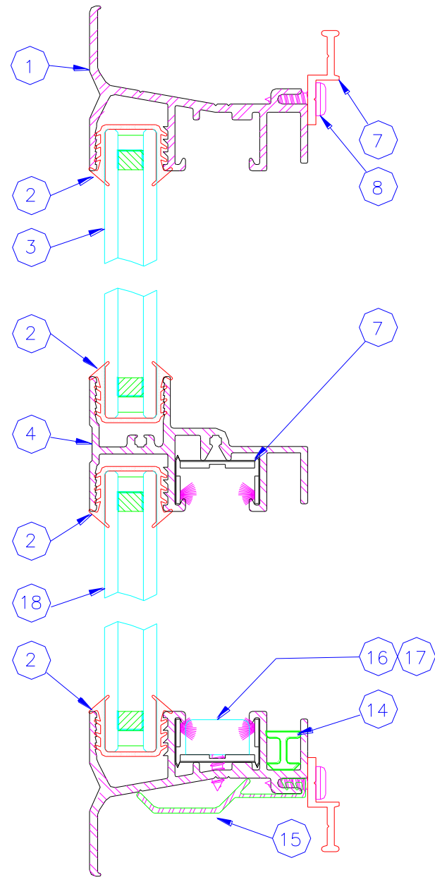
SECTION C-C
