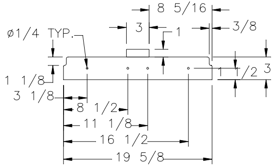
QTY: 1 MATERIAL: 3" x 1/8" FLAT
