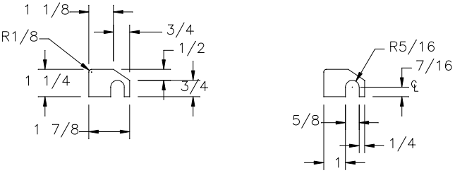
QTY: 1 SCALE: x2 MATERIAL: 3/16" FLAT
