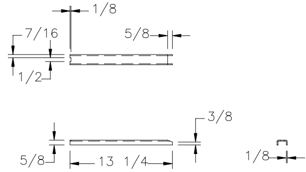
MATERIAL: 1 5/16" x 5/8" x 1/8" C-CHANNEL
