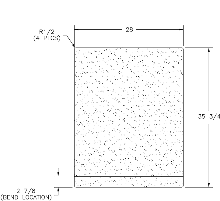
CNC PANELS
