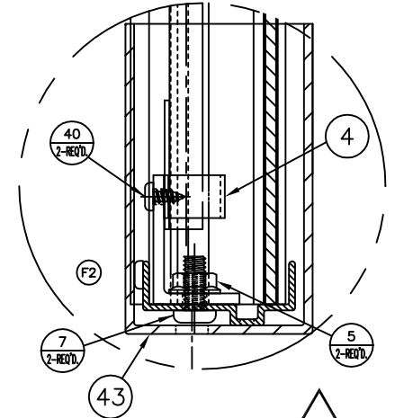
SECTION C-C SCALE : FULL
