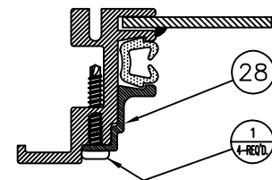
SECTION D-D SCALE : FULL
