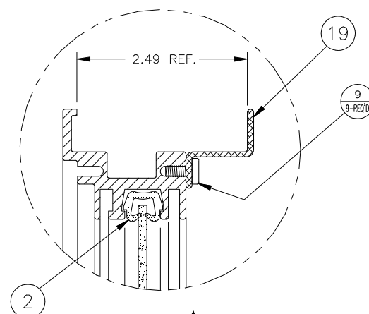
DETAIL J SCALE: FULL
