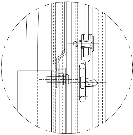
DETAIL K SCALE: FULL
