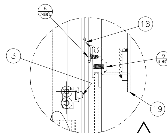
DETAIL H SCALE: FULL
