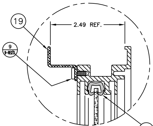
DETAIL J SCALE: FULL
