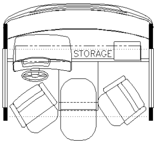
K085 - COCKPIT DINETTE
