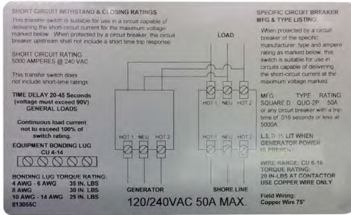
PD52 :: PROGRESSIVE DYNAMICS 50 AMP TRANSFER SWITCH :: 96122
