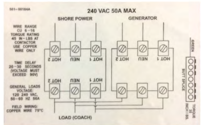
40100-001 :: TRC 50 AMP TRANSFER SWITCH :: 134638
