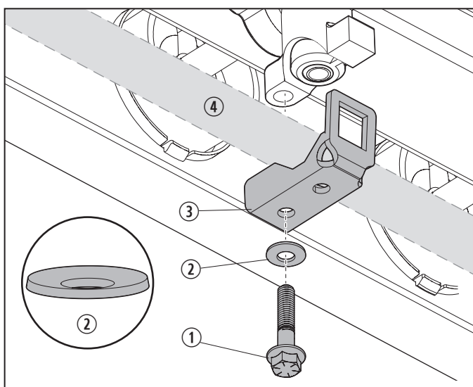
7 Install the Bell Washers
