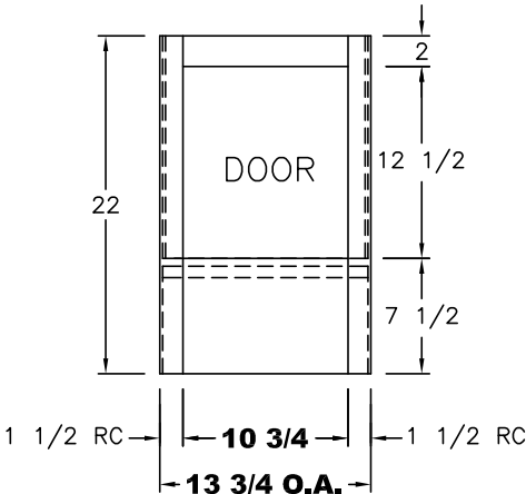
RIGHT CHEST BASE FRONT VIEW (1) 11 3/4x18 1/2 DOOR
