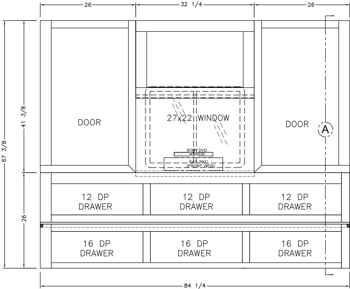
BR S-O CABINET FRONT VIEW
