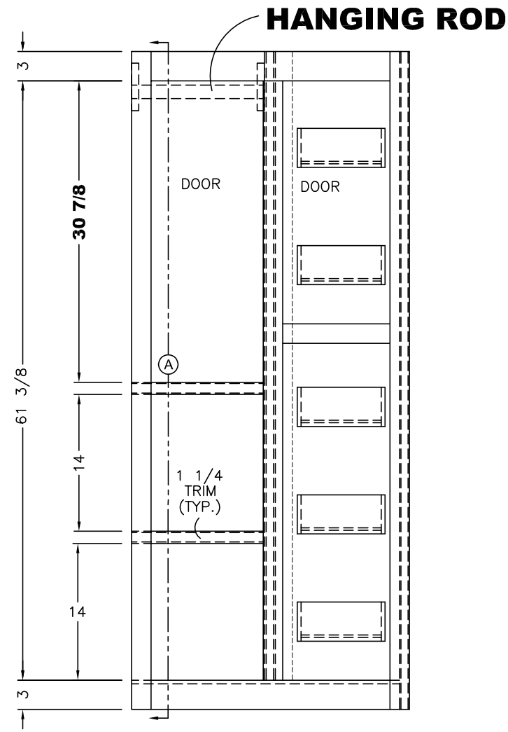
FRONT VIEW
