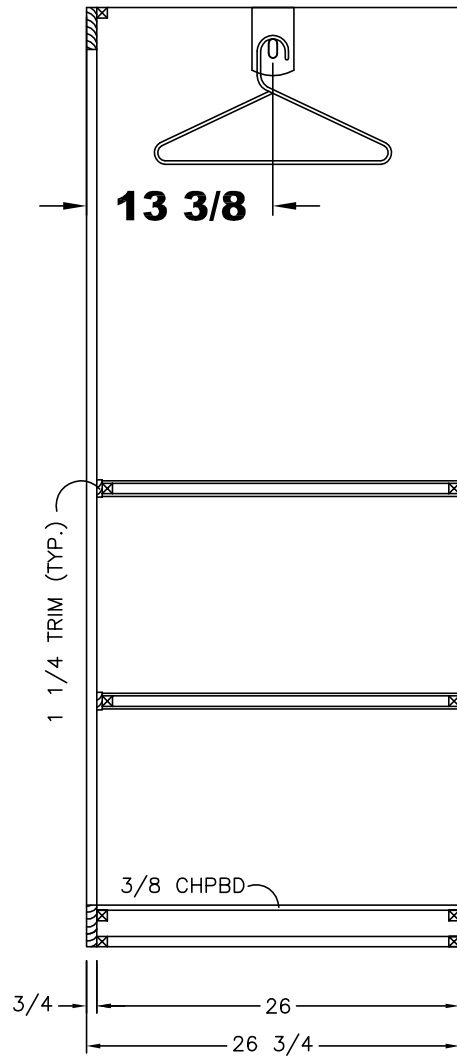
SIDE SECTION (A)
