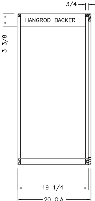
SIDE SECTION B
