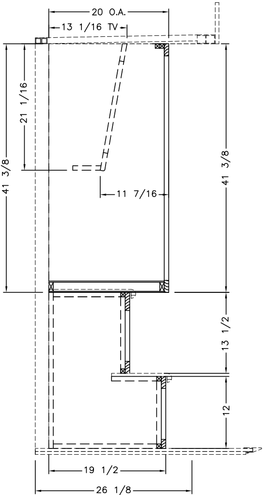
SECTION (A)
