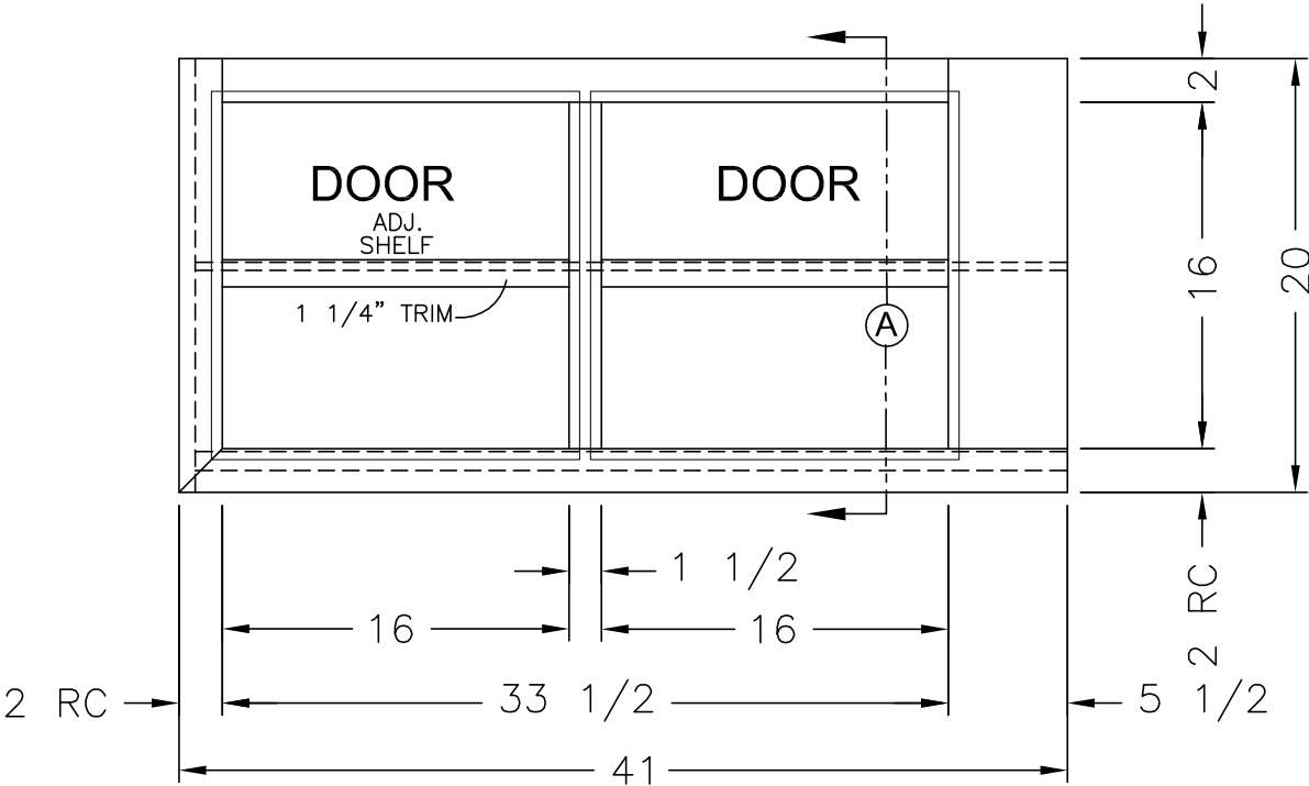
FRONT VIEW (2) 17 X 17 DOORS
