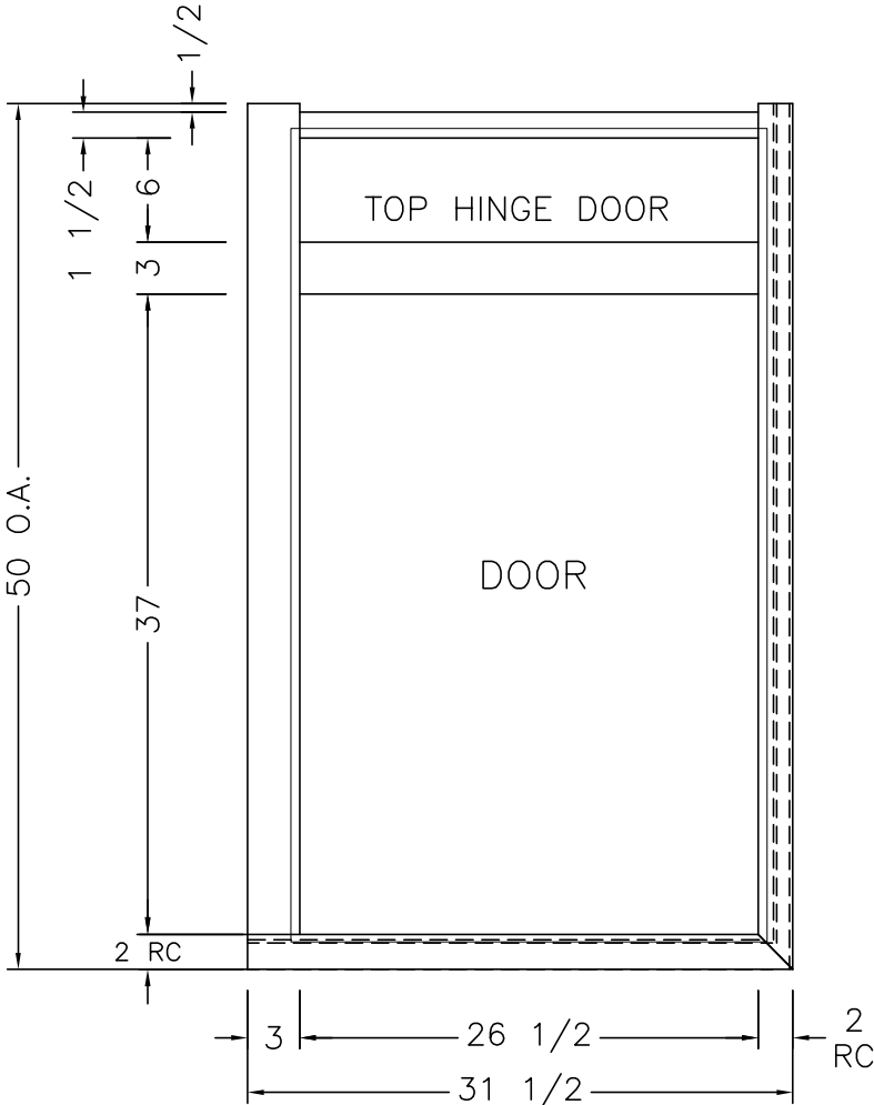
FRONT VIEW FRONT SHIRT WARD (1) 27 1/2 X 46 3/4 MIRRORED DOOR
