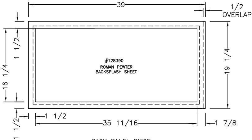
BACK PANEL PIECE 1/2" SOLID SURFACE FRAME
