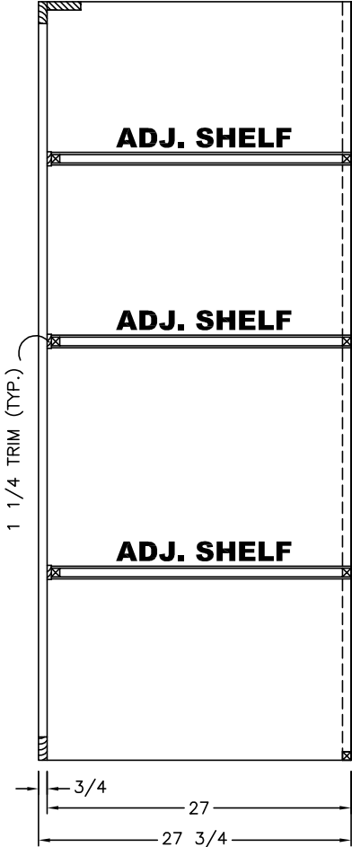
SIDE SECTION (B)
