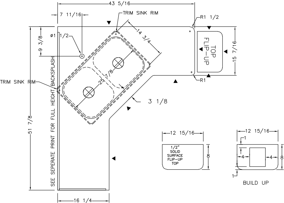
TOP VIEW KITCHEN COUNTER TOPS 1/2" SOLID SURFACE TOP ► - DENOTES A FINISHED EDGE
