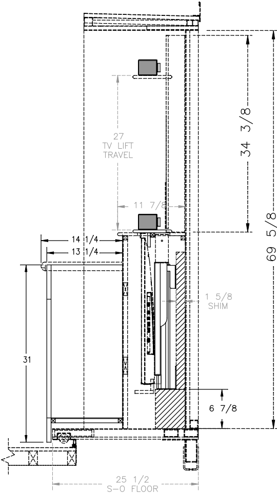
SIDE SECTION
