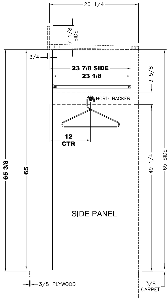
SIDE SECTION
