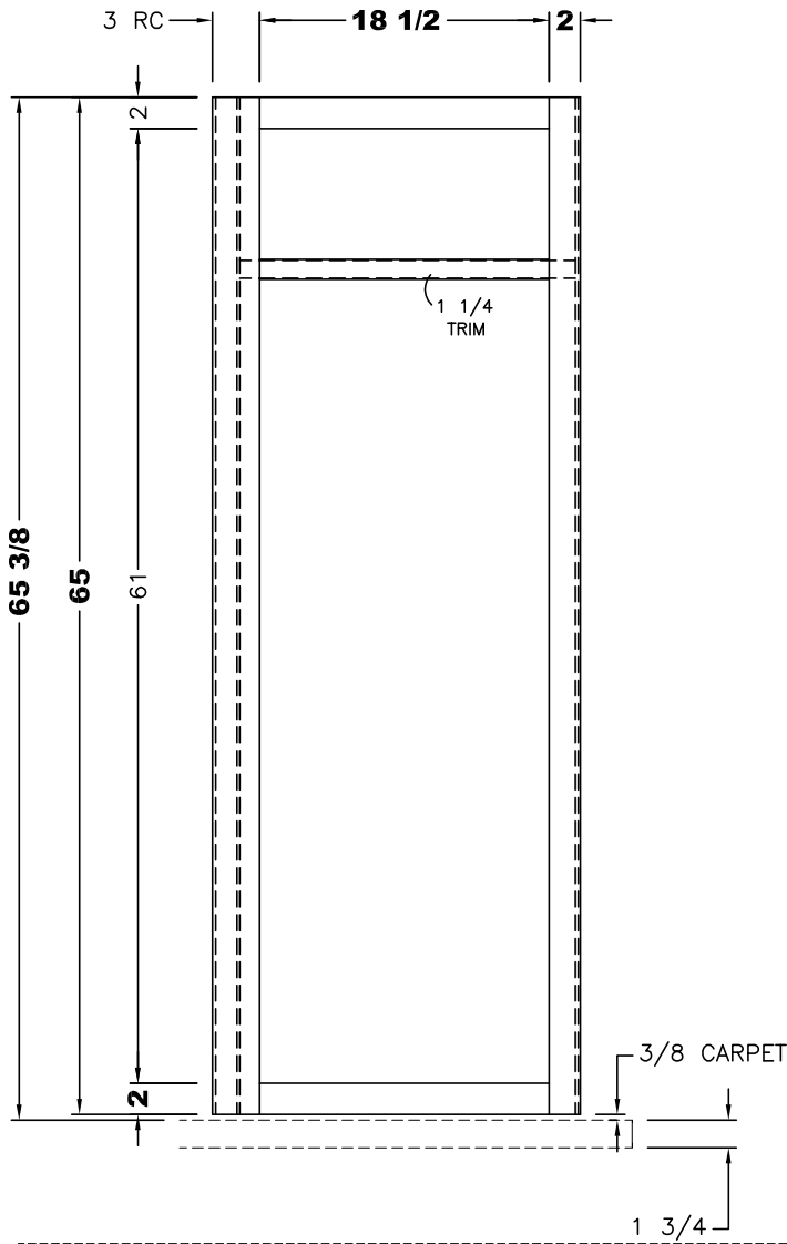
FRONT VIEW (2) 9 3/4 x 61 1/2 DOORS
