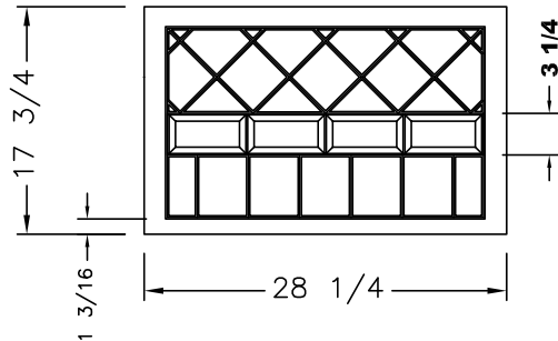
SIDE PIECE (ON REFER) MATERIAL: 1/2" SOLID SURFACE
