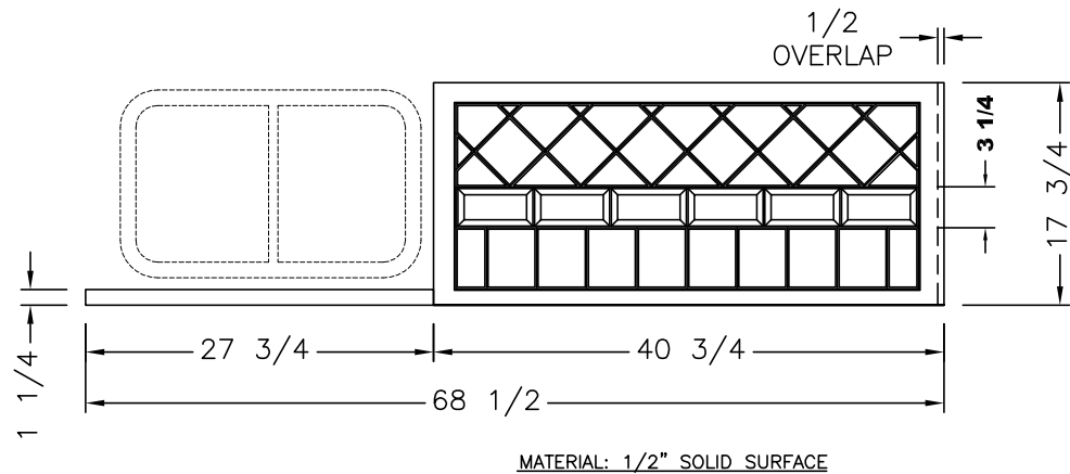
SIDE PIECE (ON S-O END WALL) MATERIAL: 1/2" SOLID SURFACE
