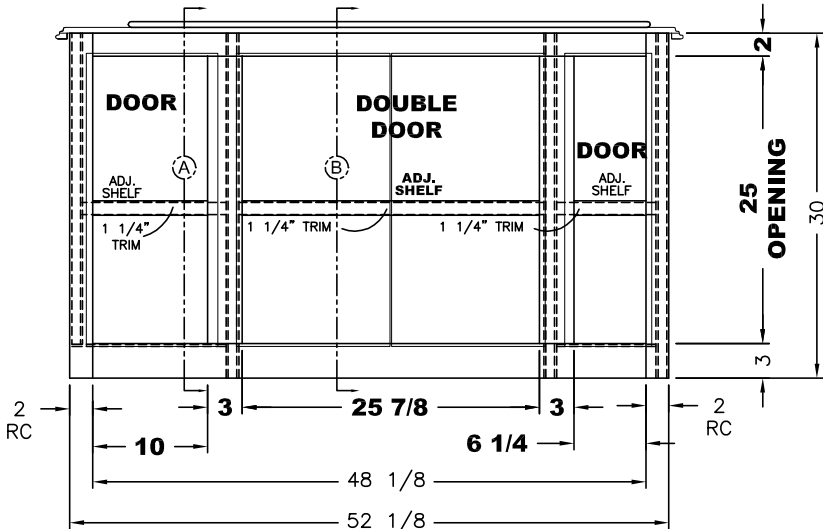
VIEW (B)
