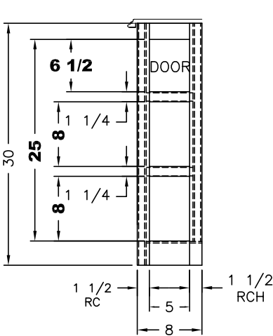
VIEW (A)
