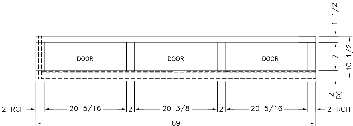
FRONT VIEW (3) 20 7/8 x 8 TOP HINGE DOORS
