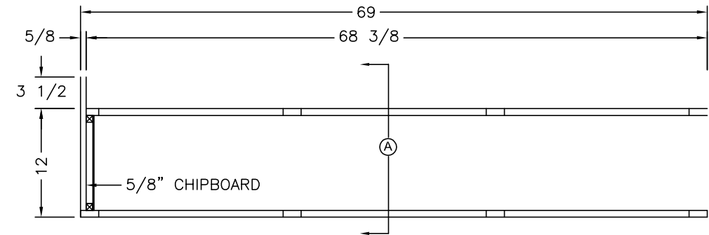
TOP VIEW OF BOTTOM PANEL
