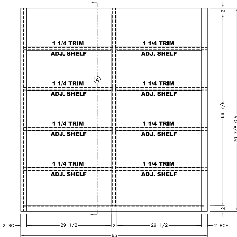
FRONT VIEW (4) 15 1/8 x 67 3/8 DOORS
