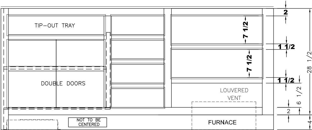
FRONT VIEW (1) 8 1/4 X 24 3/4 FRONTS
