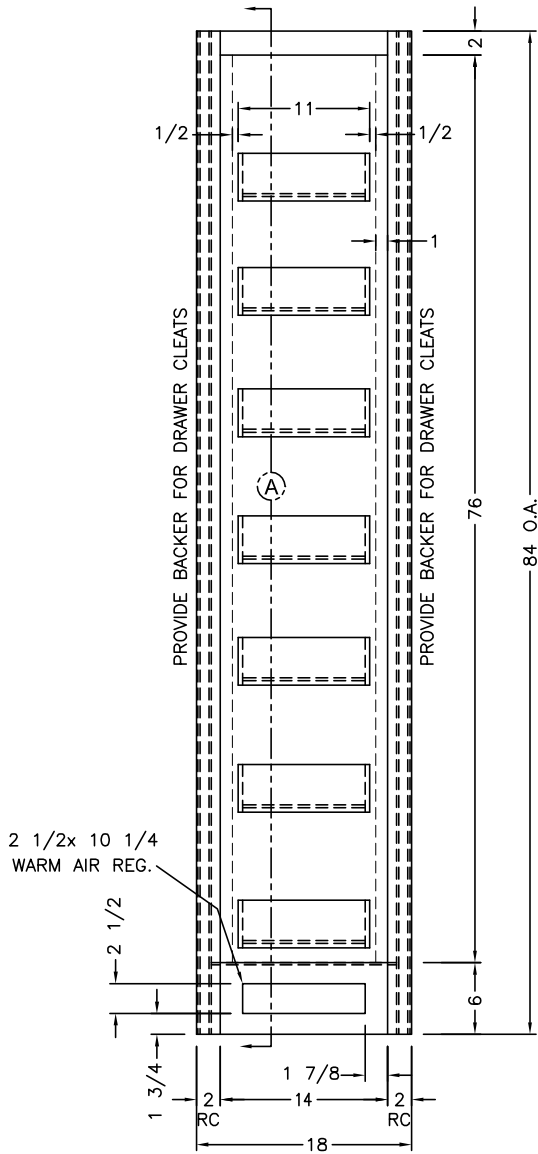
FRONT VIEW (2) 7 3/8 x 76 1/2 DOORS
