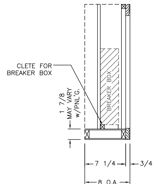
SIDE SECTION (A)
