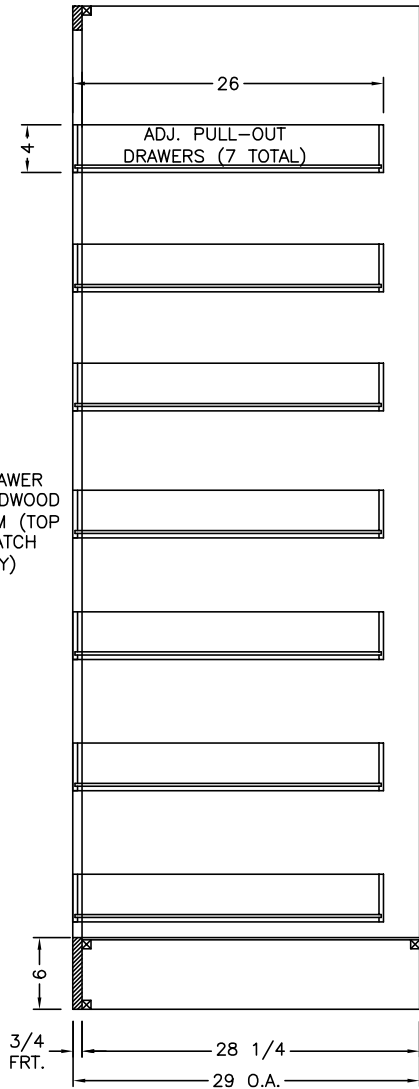
SIDE SECTION (A) W./DRAWERS
