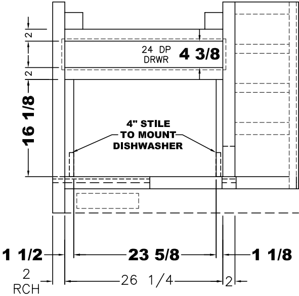
FRONT VIEW (1) 5 1/8 X 27 1/4 FRONT
