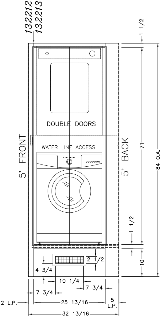
VIEW (B) (2) 13 1/4x71 1/2 LOUVERED DOORS
