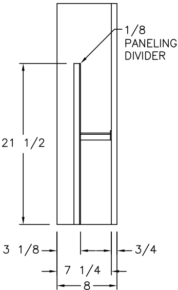
SIDE SECTION (A)
