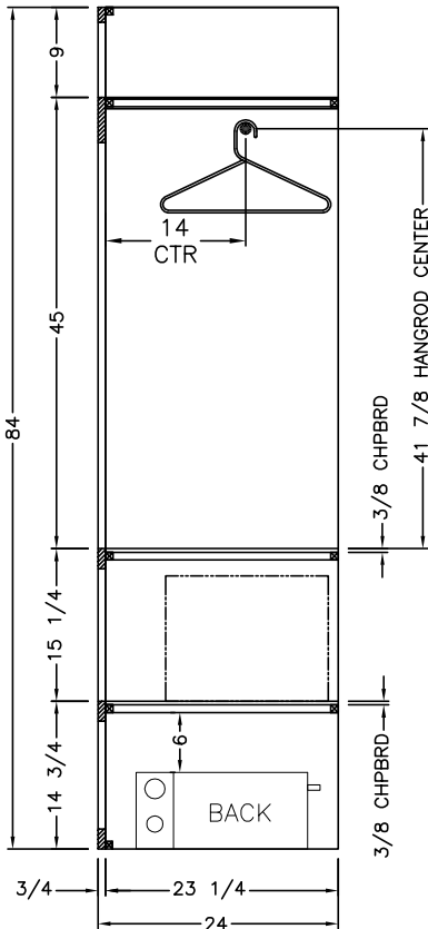
SIDE SECTION A
