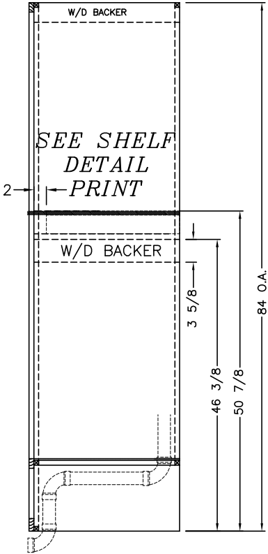
SIDE SECTION (B)
