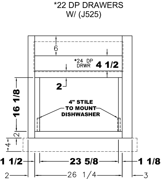
VIEW (A) (1) 9x26 3/4 FRONT
