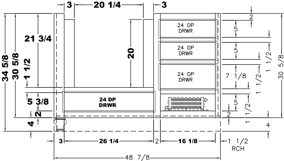
VIEW A (1) 6 1/8x27 1/4 FRONT (2) 5 3/4x17 1/8 FRONTS (1) 7 3/4x17 1/8 FRONT
