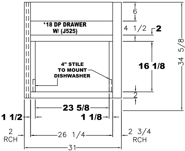
VIEW (B) (1) 9 X 27 1/4 FRONT
