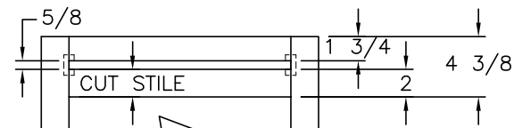
CABINET BASE FRONT VIEW
