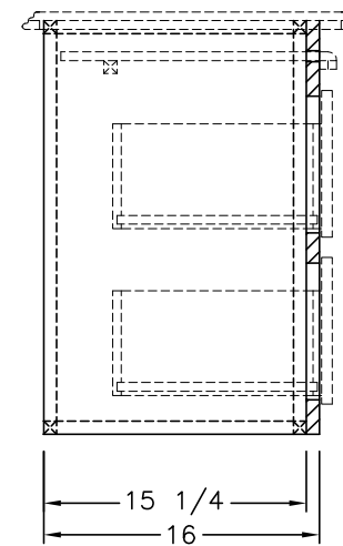
SIDE SECTION (A)
