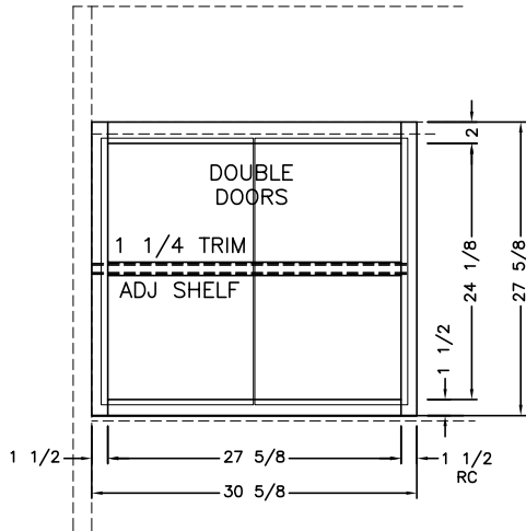
WARDROBE (2) 14 3/8 X 25 1/8 DOORS
