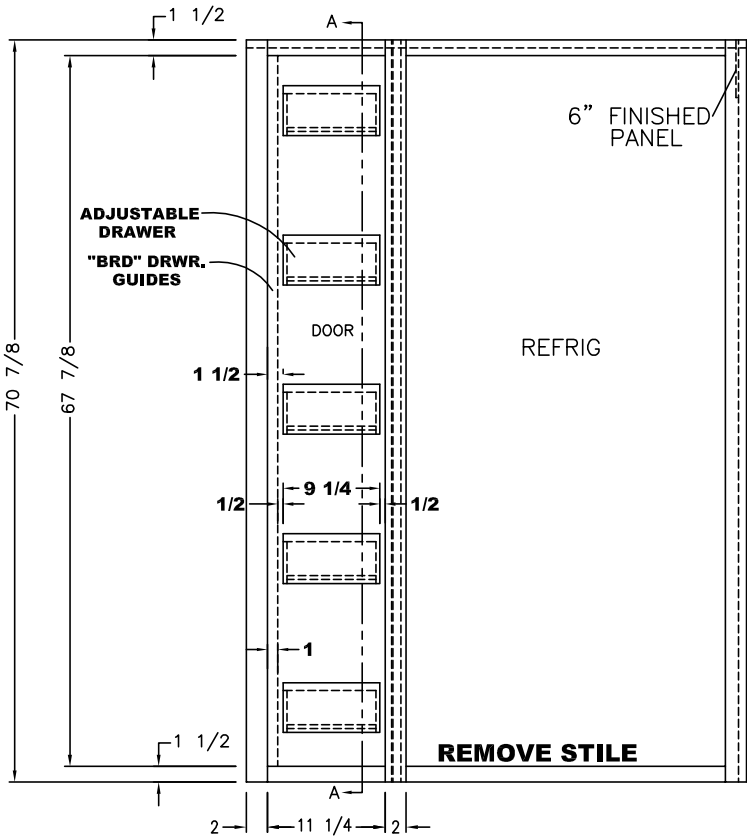
FRONT VIEW (1) 12 1/4x68 5/8 DOOR
