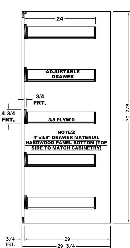
SECTION VIEW A-A
