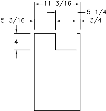
CHEST TOP 1/2" SOLID SURFACE ▶ - DENOTES A FINISHED EDGE
