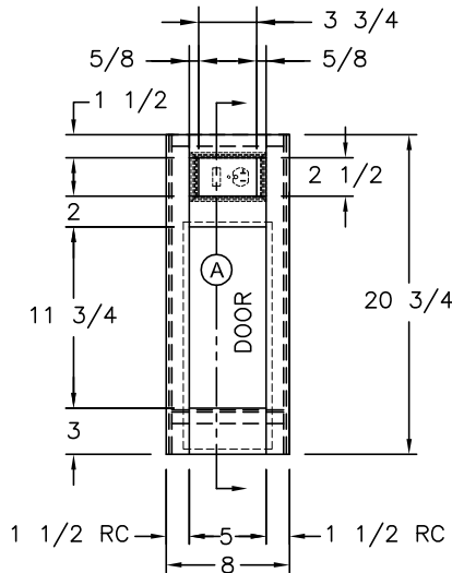
(1) 6x14 3/4 DOOR (LARGER OVERLAP AT BOTTOM)
