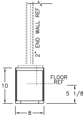
REAR CHEST TOP VIEW
