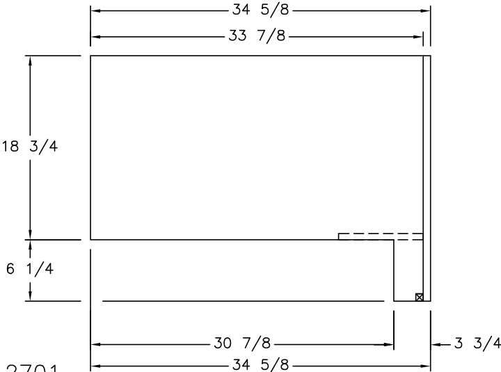
RT SIDE VIEW
