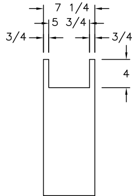
BACK PANEL
