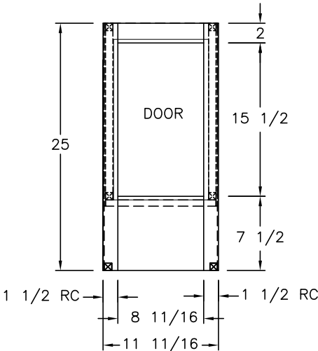
(1) 16 1/4x9 5/8 DOOR
