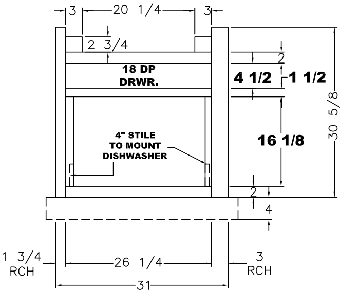
VIEW ⓑ (1) 5 1/8 X 27 1/4 FRONT
