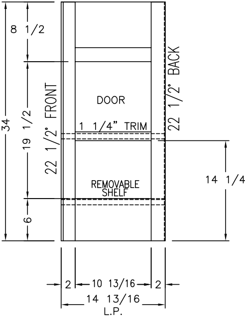
VIEW (B)
