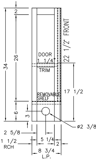
VIEW (A)
