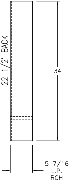
VIEW (C)
