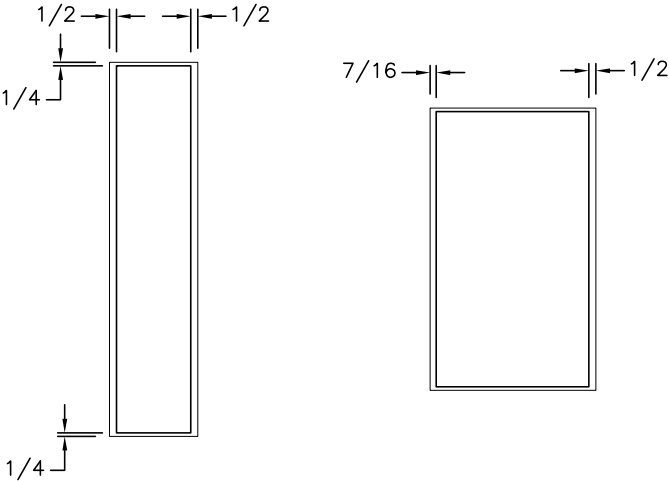
DOOR OVERLAPS
