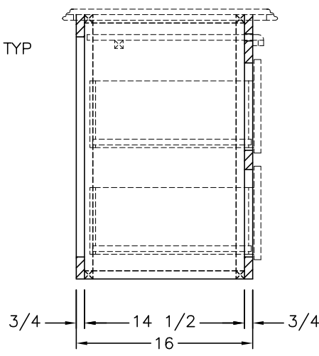
SIDE SECTION (A)
