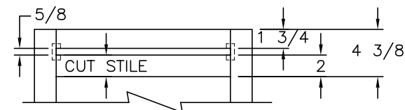
CABINET BASE FRONT VIEW
