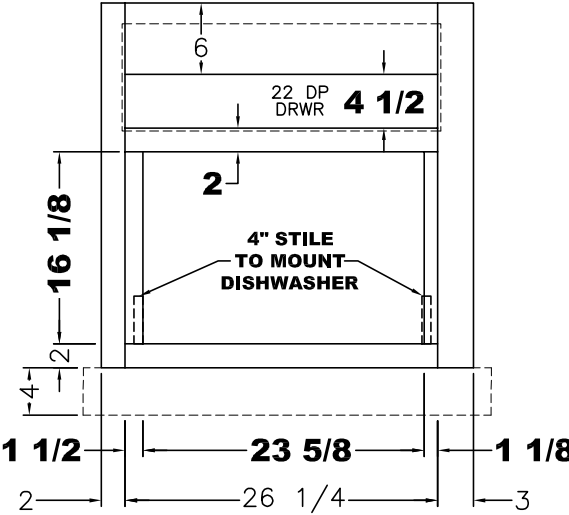
VIEW (A) (1) 9x26 3/4 FRONT
