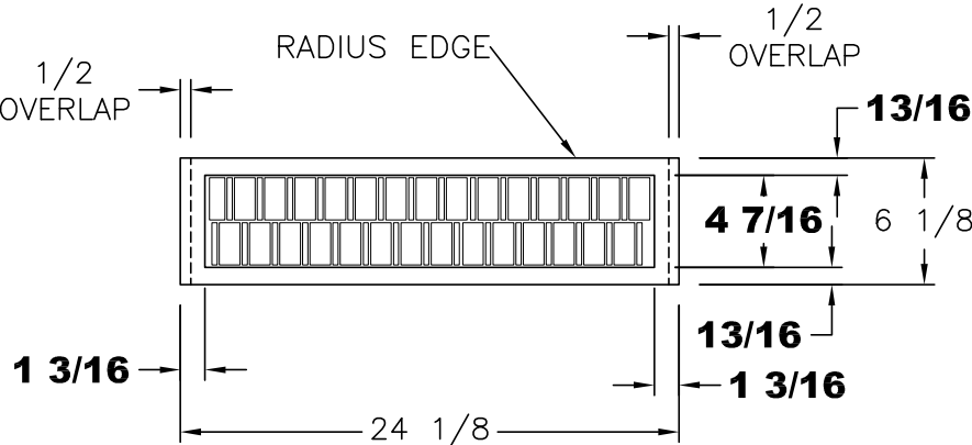
VIEW B
