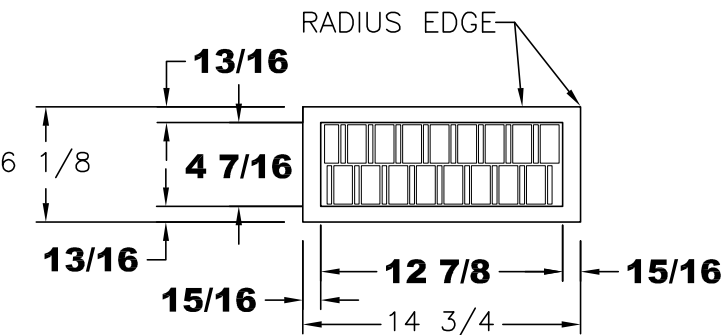
VIEW C
