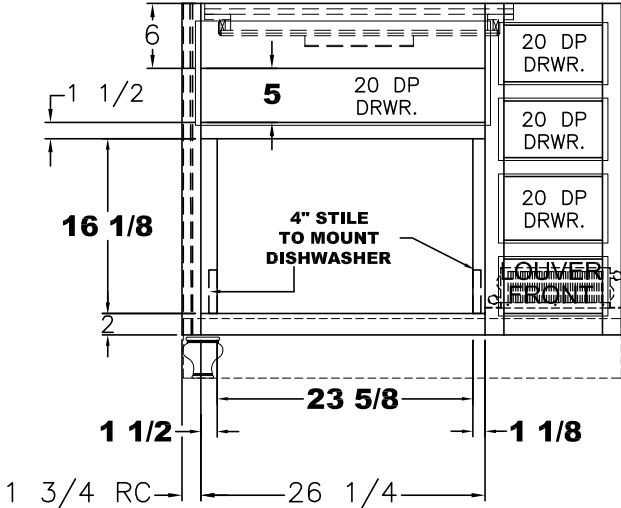
VIEW (A) J550 (1) 9 5/8x27 1/4 FRONT (2) 5 3/4x10 1/8 FRONTS (1) 6 3/8x10 1/8 FRONT
