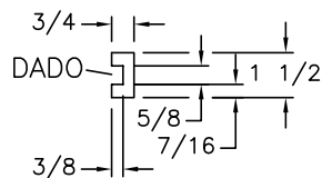
HARDWOOD TRACK DETAIL
