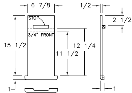
1/2 SOLID SURFACE P-O SHELF
