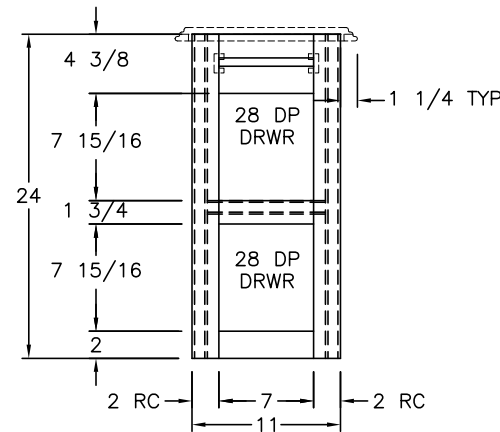
FRONT VIEW (2) 7 1/2x8 1/2 FRONTS
