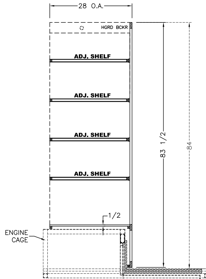
SIDE SECTION B
