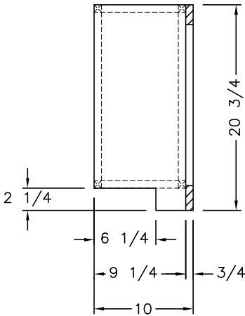
SIDE SECTION (A)
