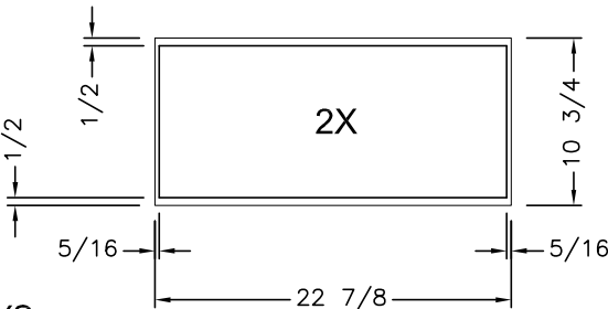
FRONT VIEW (2) 22 7/8 X 10 3/4 DOORS (TOP HINGE)
