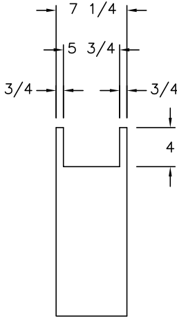
BACK PANEL
