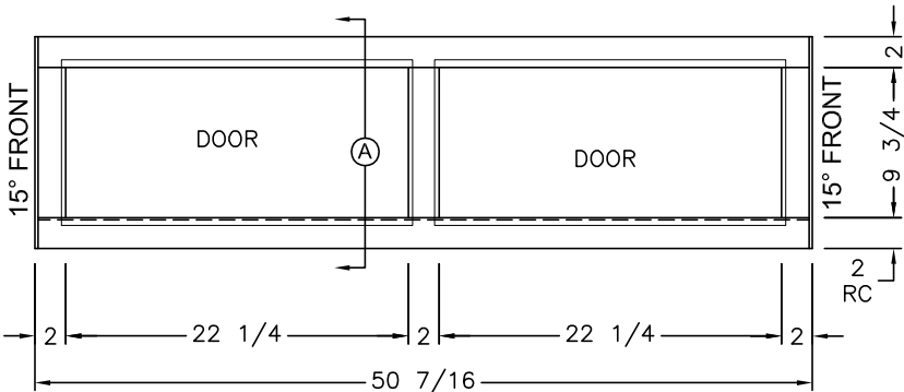
FRONT VIEW (2) 22 7/8 X 10 3/4 DOORS (TOP HINGE)
