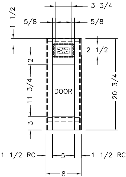
(1) 6x14 3/4 DOOR (LARGER OVERLAP AT BOTTOM)
