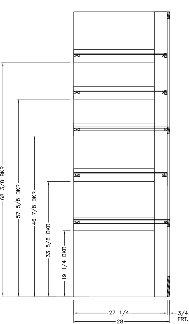
SECTION A
