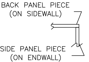
INSTALLATION DETAIL (SCALE 4X)
