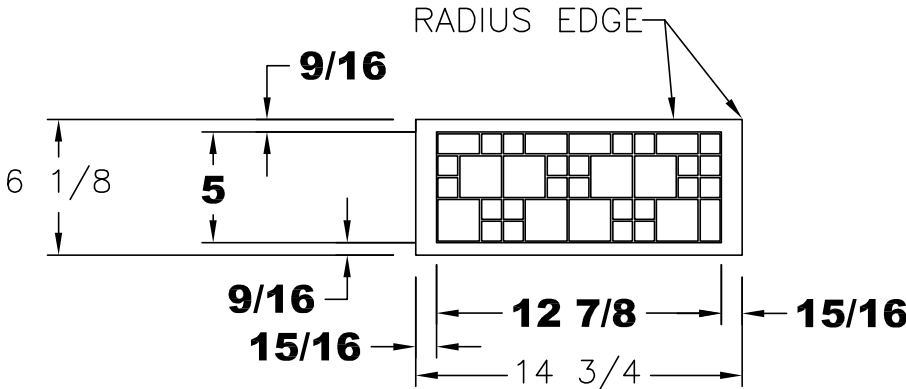
VIEW C
