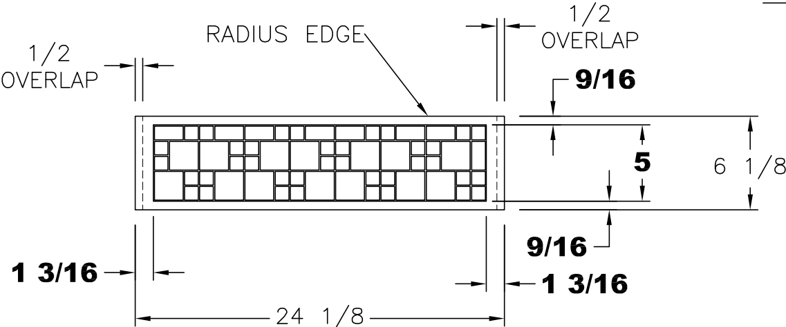
VIEW B
